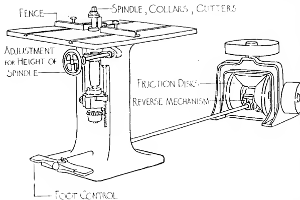
FIG. 197. SHAPER.
